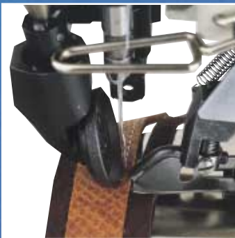
Edge trimming device, operated from below. Machines can be used for standard sewing with needle size up to 160.
